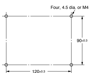
Mounting Holes
