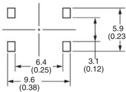
PCB Pad (Top View) (One-side PCB t= 1.6)
