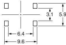
PCB Pad (Top View) (One-side PCB t= 1.6)
