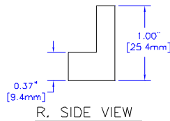
MOUNTING FEET DETAIL
