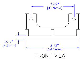
MOUNTING FEET DETAIL
