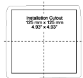
Installation Cutout
