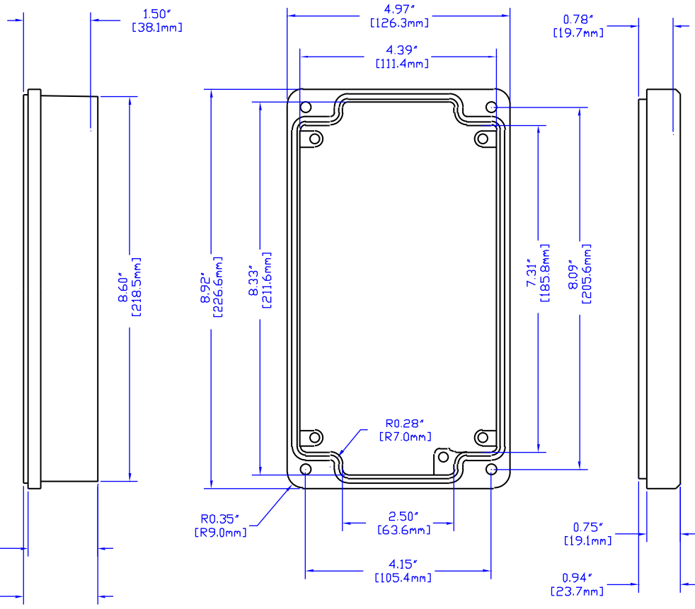
VIEW OF LID (INSIDE)
