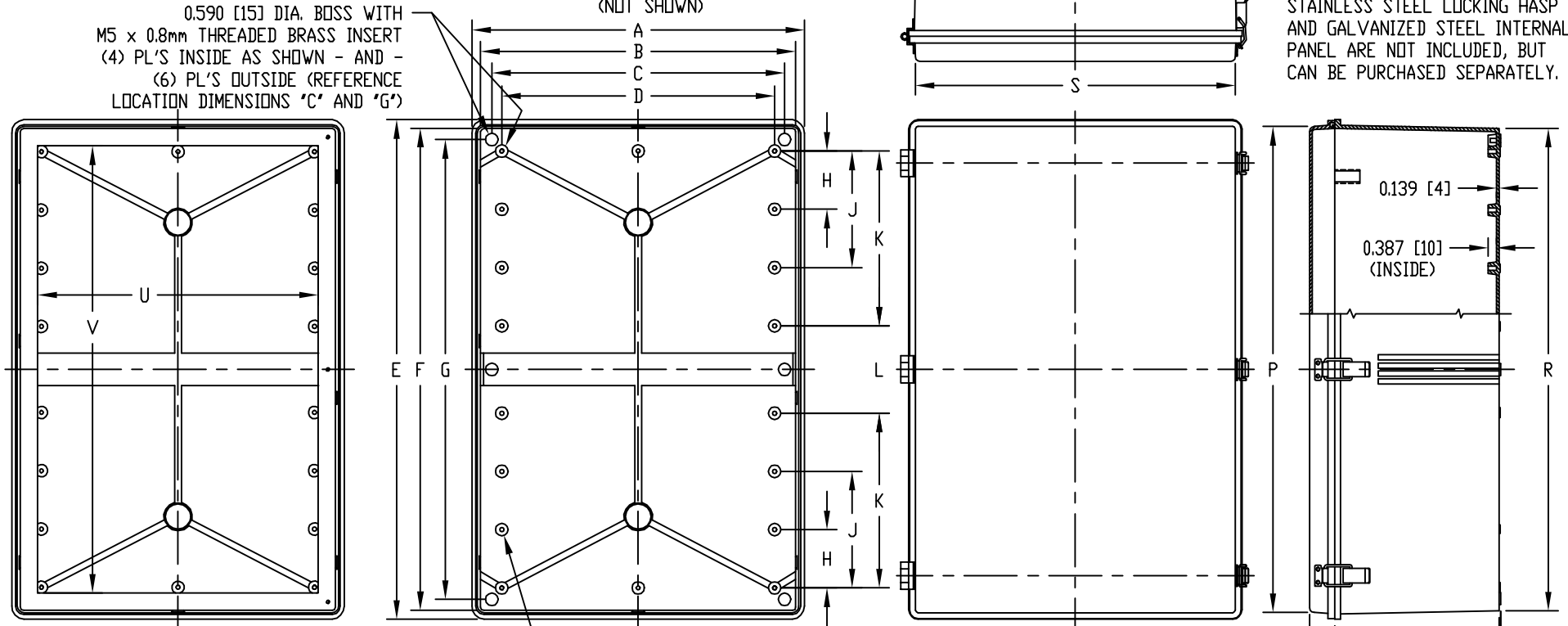
VIEW LESS COVER 0.590 [15] DIA. BOSS WITH 0.197 [5] DIA. HOLE x 0.410 [10] DEEP AND PANEL MOUNTING FRAME (14) PLACES
