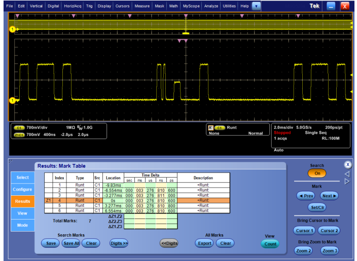
Search – Results of an advanced search for a runt pulse within a long waveform record. Each instance of the runt is automatically marked for easy reference. Wave Inspector controls provide unprecedented efficiency in viewing and navigating waveform data.
