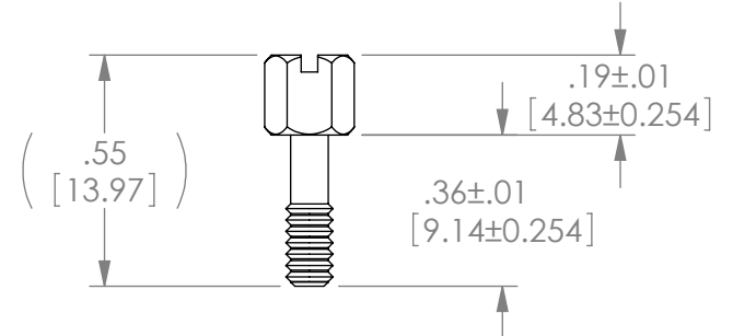
JACKSCREW SPECIFICATION
