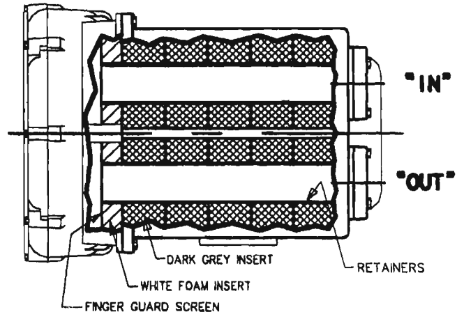
VIEW - LOOKING DOWN AT TOP OF BLOWER (MOTOR REMOVED FOR CLARITY)
