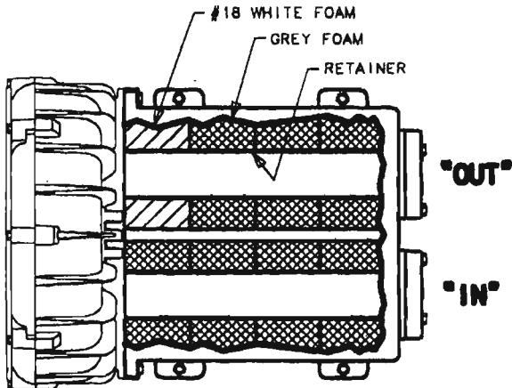
VIEW - LOOKING DOWN AT TOP OF BLOWER (MOTOR REMOVED FOR CLARITY)
