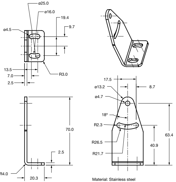
Side-mount Mounting Bracket Model OMH-ML17-1 for ML17 Series sensors
