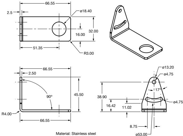
Snout-mount Mounting Bracket Model OMH-ML17 for ML17 Series sensors
