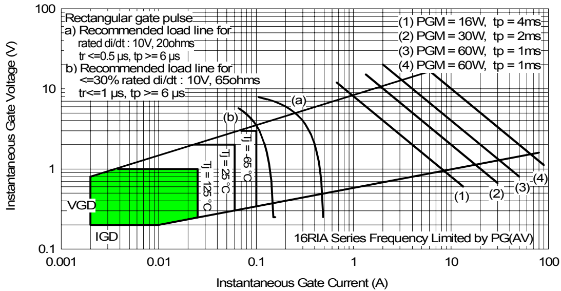
Fig. 16 - Gate Characteristics
