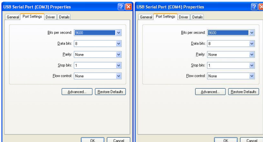
Figure 2.9 - Settings Tab
