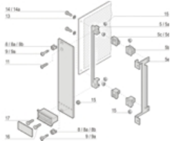
Item 13, 3 U front panel mounting
