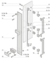
Item 13, 6 U front panel mounting
