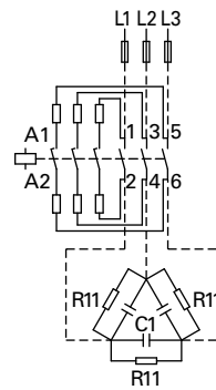
Power Circuit—11–85 kVAR
