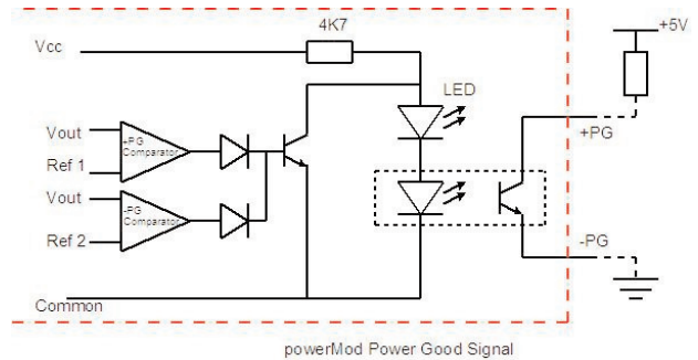
powerMod Power Good Signal
