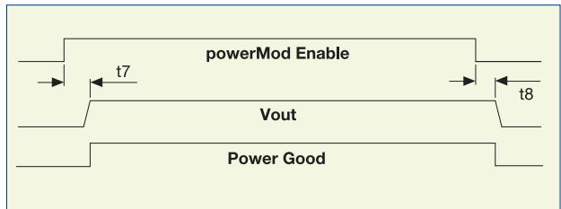
powerMod Power Good Signal
