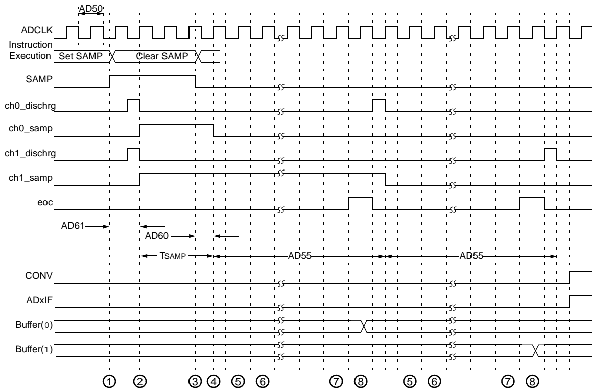
FIGURE 23-18: A/D CONVERSION (10-BIT MODE) TIMING CHARACTERISTICS (CHPS<1:0> = 01, SIMSAM = 0, ASAM = 0, SSRC<2:0> = 000)
