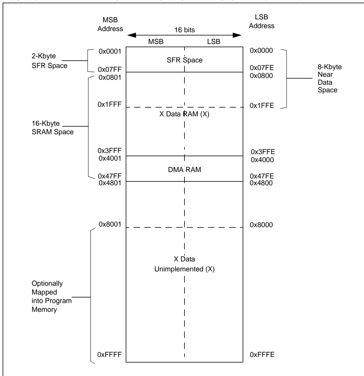
FIGURE 3-4: DATA MEMORY MAP FOR PIC24H DEVICES WITH 16 KBYTES RAM
