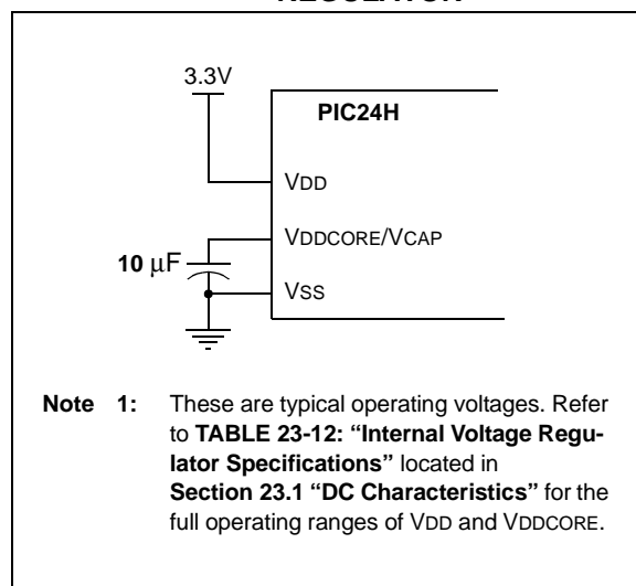
FIGURE 20-1: CONNECTIONS FOR THE ON-CHIP VOLTAGE REGULATOR (1)
