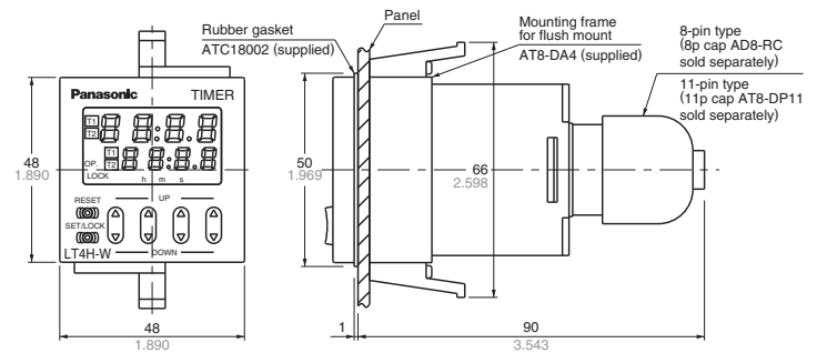
Pin type
