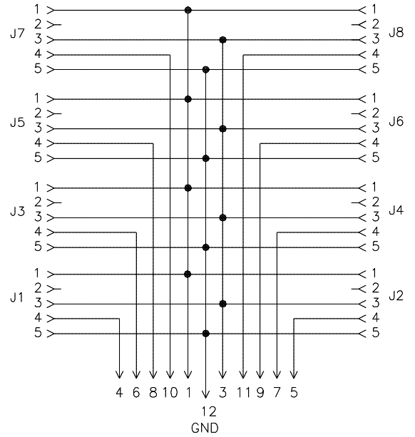
WIRING DIAGRAM
