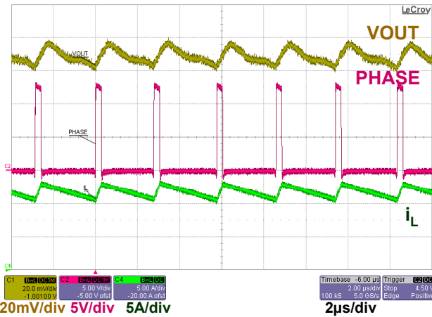
Figure 11: CCM ( I_{OUT} = 12A )
