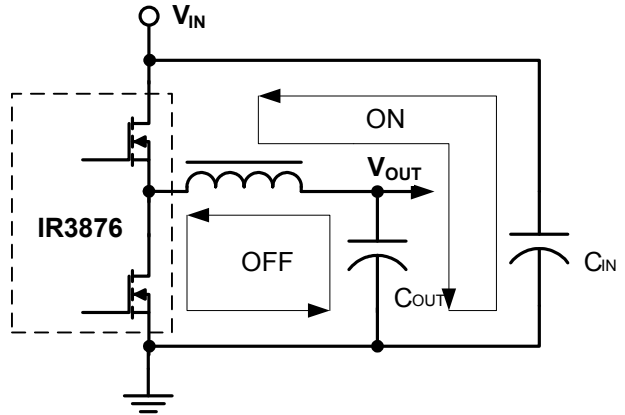
Figure 20. Current Path of Power Stage
