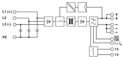
Block diagram
