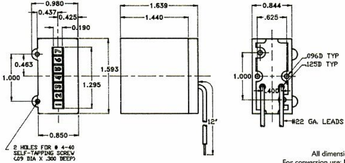
Series E14B Back of Panel or Rear Mount
