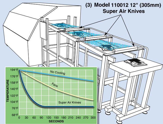
PVDF Super Air Knives provide superior corrosion resistance.
