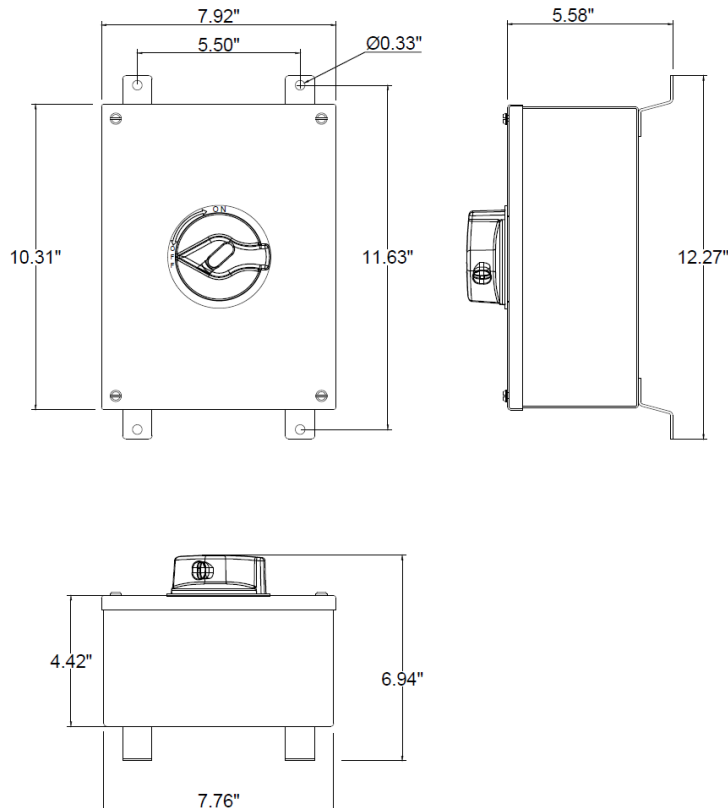
Drawing Not to Scale
