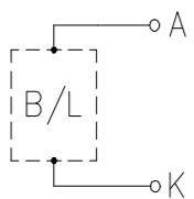
CONSTANT CURRENT: 30mA, (VF: MIN2.9V, TYP3.0V, MAX3.2V) BACKLIGHT DRIVER CIRCUIT DIAGRAM
