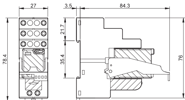
Type 58.34 Screw terminals
