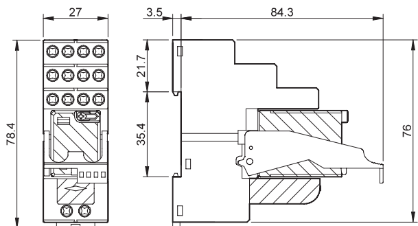
Type 58.P3 Push-in terminals
