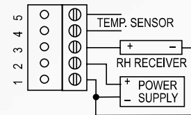
Models with 0-5 or 0-10 V RH output and a passive thermistor temperature sensor
