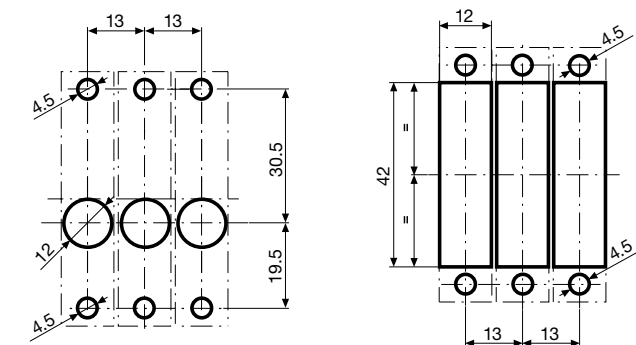
Installation from rear
