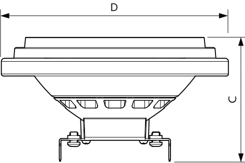
16AR111/LED/927/F40/DIM/EC 12V 6/1FB
