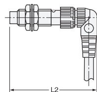
L-shape Connectors
