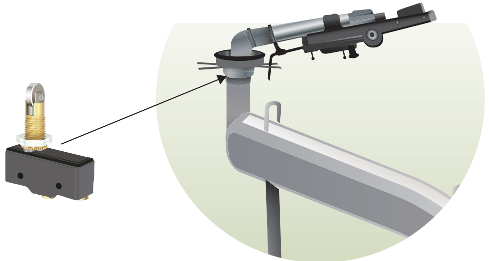
Figure 2. MICRO SWITCH BZ Switches in the End Gun
