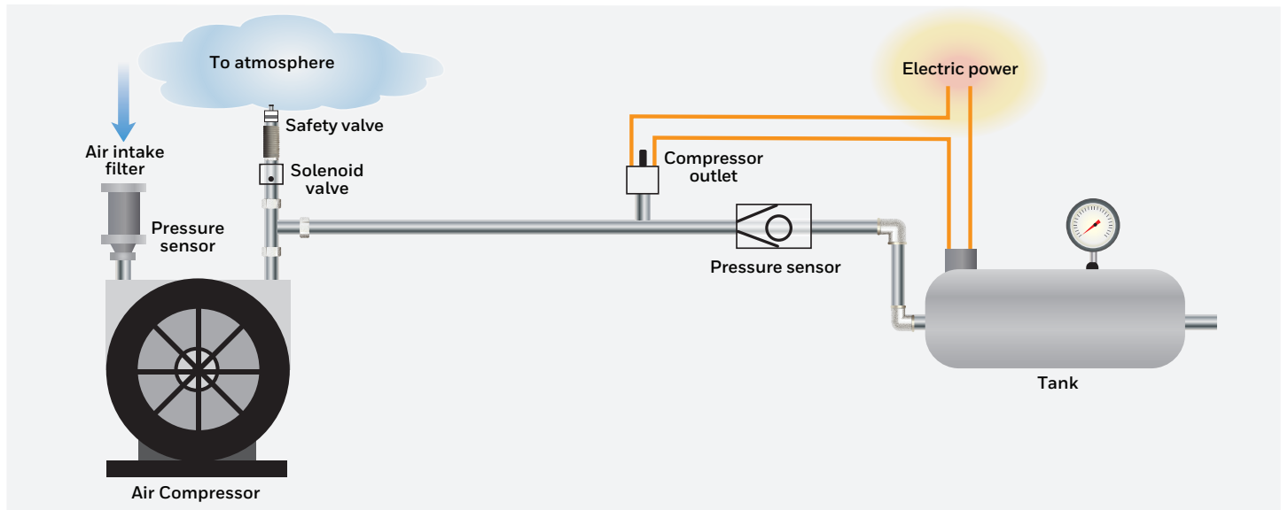
FIGURE 2: HEAVY-DUTY PRESSURE TRANSDUCERS USED IN AIR COMPRESSORS
