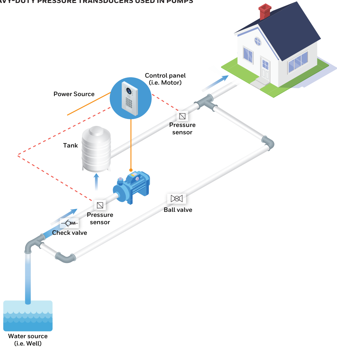
FIGURE 1: HEAVY-DUTY PRESSURE TRANSDUCERS USED IN PUMPS
